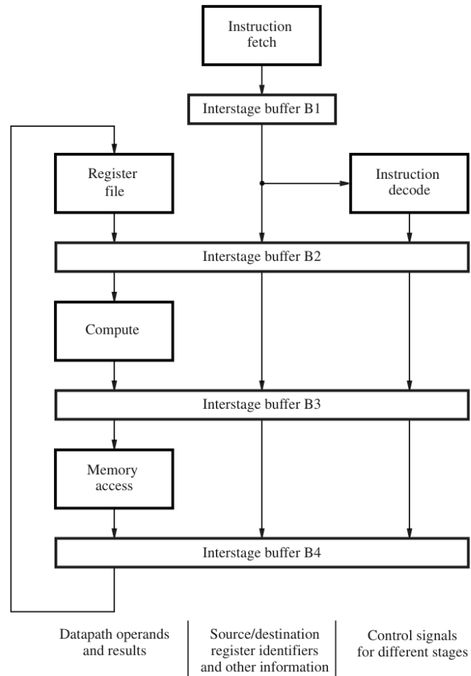
Figure 6.2 A five-stage pipeline.
