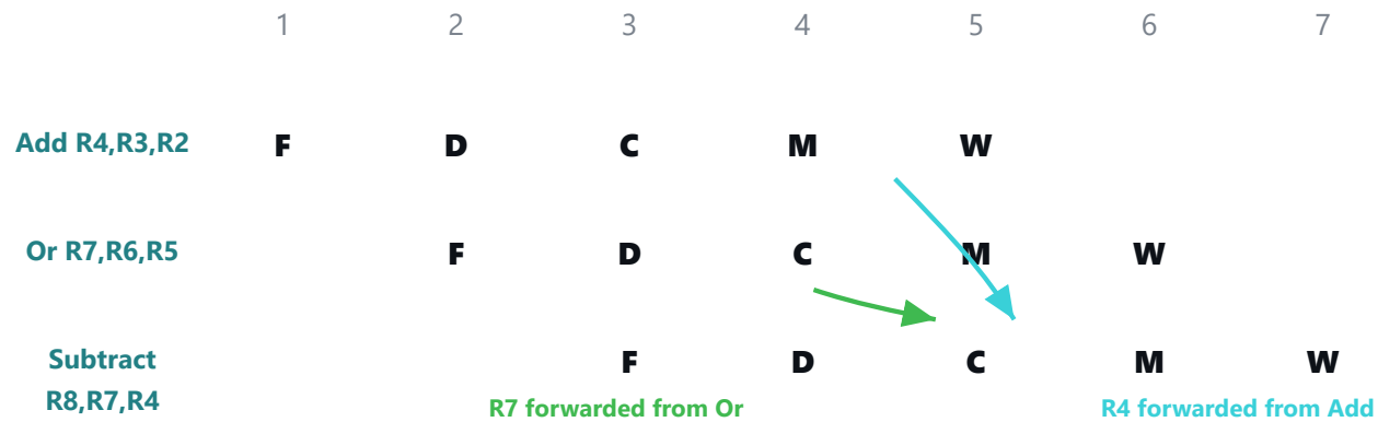
Figure 6.15 — Two operands forwarded into one instruction; no stall required.
