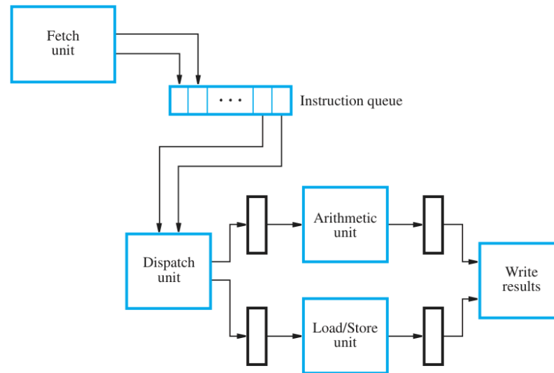
Figure 6.13 A superscalar processor with two execution units.
