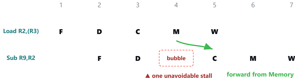
Figure 6.8 — A load-use hazard: forwarding still needs a single-cycle stall.
