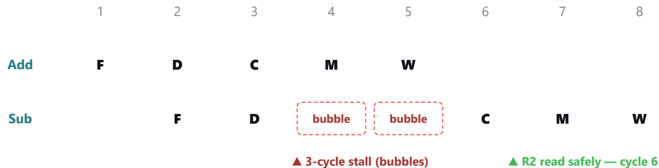
Figure 6.3 — Pipeline stall due to a data dependency (3-cycle stall).
