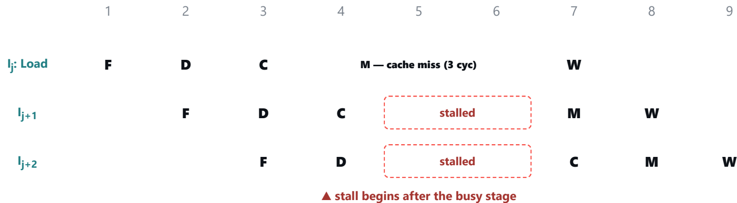
Figure 6.7 — Stall caused by a memory access delay for a Load instruction (drawn for a 3-cycle delay; a real cache miss costs 10+).
