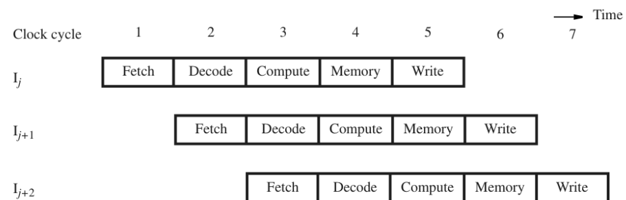
Figure 6.1 Pipelined execution—the ideal case.
